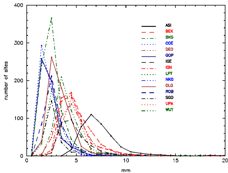
Fig. 4: Histogram of site-specific standard deviations (GPS weeks 1143-1159)
