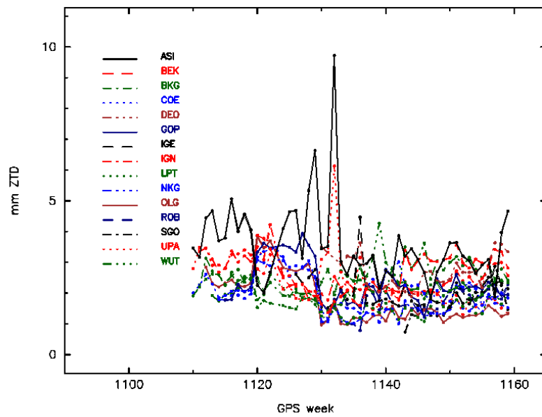
Fig. 2: Standard deviation of the weekly mean biases
